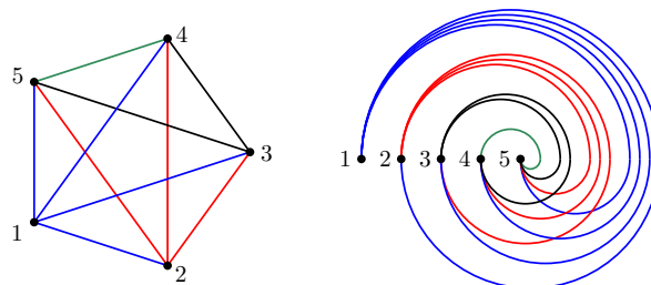
■ Figure 4 (left) the perfect convex C_5 and (right) the perfect twisted drawing T_5 .
