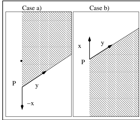
Figure 1: Shells of 3 \times 3 H -normal matrices of type 3
