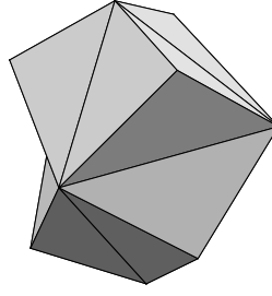
Figure 5. A discrete Willmore sphere of noninscribable type with 11 vertices and W = 2\pi .
