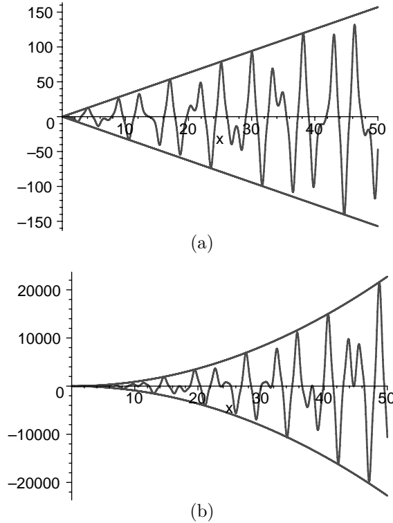
FIGURE 5. Two directional derivatives of the Riemann theta function \theta(0, ix|\Omega) with \Omega as in (22). As before, the exponential growth-factor has been factored out. In (a) the directional derivative of order one with \mathbf{k} = (1, 0) is shown, and (b) illustrates the quadratic growth of the directional derivative of order two, with \mathbf{k}^{(1)} = \mathbf{k}^{(2)} = (1, 0) .
