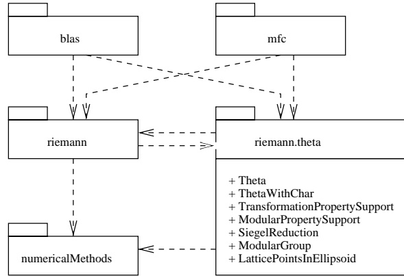
FIGURE 7. Dependencies of the package riemann.theta .
