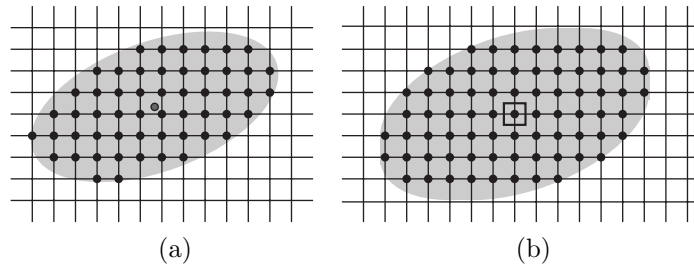
FIGURE 3. Summation indices (in black) (a) for a pointwise approximation, inside an ellipsoid centered at [[\mathbf{Y}^{-1}\mathbf{y}]] (in grey), and (b) for a uniform approximation, inside an ellipsoid whose center moves around the unit cube.
