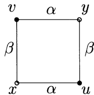
Figure 1. An elementary quadrilateral.
