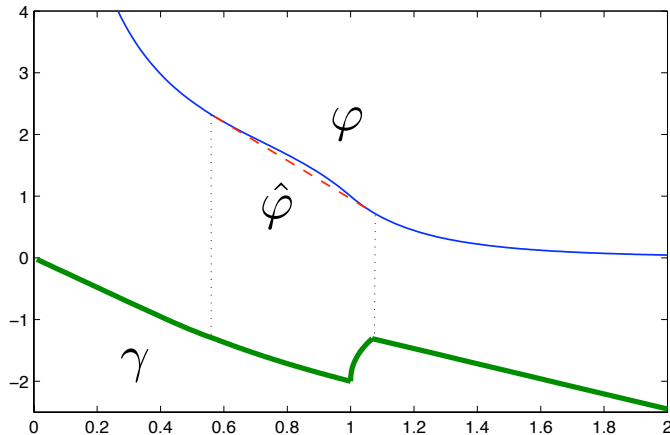
FIGURE 1. The function \varphi (solid line), its convex envelope \hat{\varphi} (dashed line) and the universal stopping signal \gamma (bold line) for the parameters r = 0.05 , \sigma = 0.15 , c = 1 .
