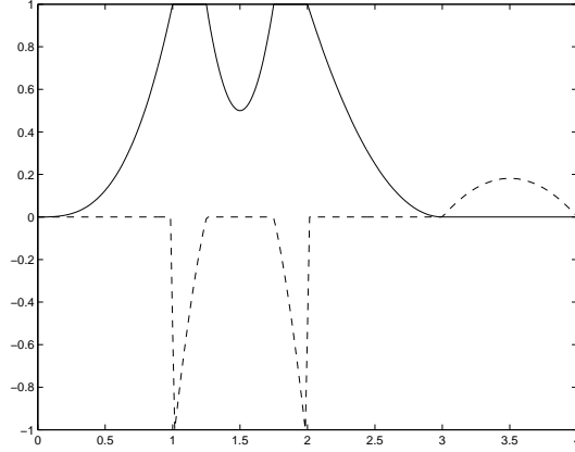
FIG. 5.1. solid: \bar{u}(x_1, x_2) , dashed: \tilde{d}(x_1, x_2)
