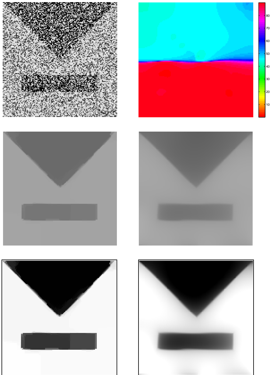
Figure 5: Top left: noisy image. Top right: smoothed rotation angles used to generate the final image on the left with parameters \mu = 10000 and \sigma = 1.5 . The smoothed rotation angles belonging to the anisotropic diffusion look very similar. Middle left: denoised image by quadratic programming with \lambda = 150 and \nu = 0.1 without rescaling. Middle right: denoised image by anisotropic diffusion with \varepsilon^2 = 0.5 , time step size \tau = 0.1 , number of iterations \text{itmax} = 1700 and \nu = \frac{1}{300} without rescaling. Bottom: same as in the middle with identical rescaling.
