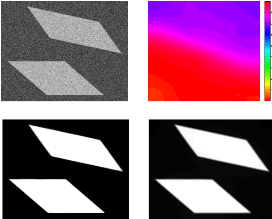
Figure 3: Top left: noisy image containing sheared rectangles with fixed shear parameter s = 0.92 and white Gaussian noise of standard deviation 50. Top right: smoothed rotation angles used to denoise the image with parameters \mu = 300000 and \sigma = 1.5 . Bottom left: denoised image by quadratic programming with \lambda = 150 and \nu = 0.04 . Bottom right: denoised image by anisotropic diffusion with \varepsilon^2 = 0.001 , time step size \tau = 0.1 , number of iterations \text{itmax} = 1800 and \nu = 0.01 .
