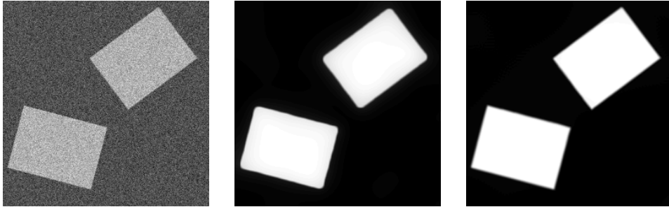
Figure 1: Left: noisy image corrupted by white Gaussian noise with standard deviation 50. Middle: denoised image using edge enhancing diffusion, see [16]. Right: denoised image using the method proposed in this paper.
