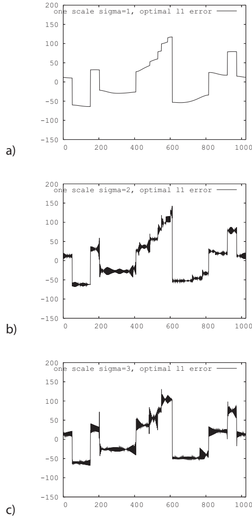
Fig. 9.a Denoising results with presmoothed diffusion and one single scale \sigma . Results with optimal \ell^1 -error. a) \sigma = 1 . b) \sigma = 2 . c) \sigma = 3 .
