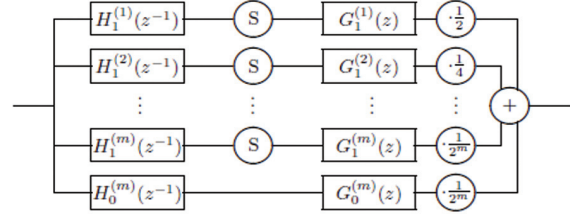
Fig. 3. Filter bank for translation invariant wavelet shrinkage, written with multiple channels.
