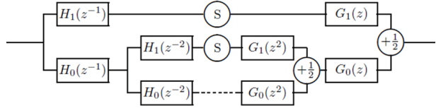
Fig. 2. Filter bank for translational invariant wavelet shrinkage with multiple scales using the algorithme à trous
