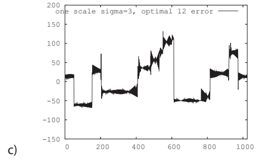
Fig. 9.b Denoising results with presmoothed diffusion and one single scale \sigma . Results with optimal \ell^2 -error. a) \sigma = 1 . b) \sigma = 2 . c) \sigma = 3 .
