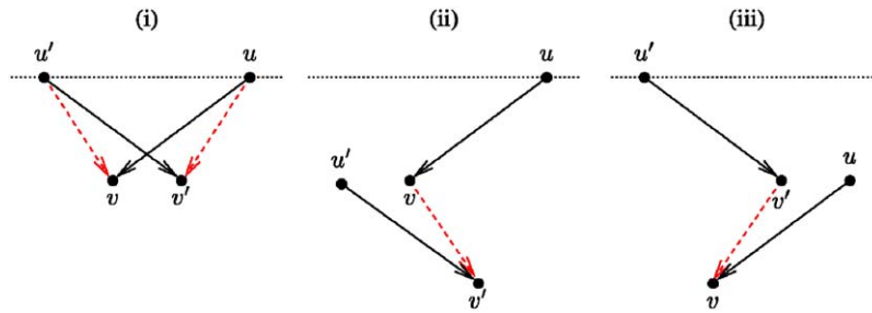
Fig. 2. An illustration of the three cases occurring in the proof of Lemma 1.
