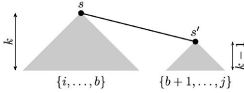
Fig. 1. The figure explains the structural result described in part (i) of Lemma 1. An optimum k -hop tree splits the set of vertices \{i, \dots, j\} into two subsets \{i, \dots, b\} and \{b + 1, \dots, j\} .
