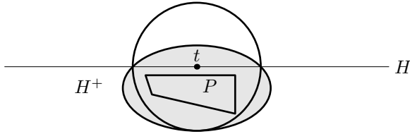
FIGURE 3. The Löwner-John ellipse of a half-ellipse.
