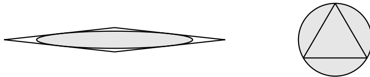
FIGURE 1. Maximal inscribed ellipse of a flat diamond, and minimal circumscribed ellipse (circle) of a regular triangle.
