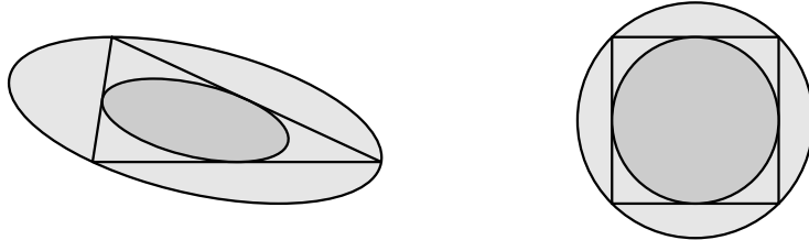
FIGURE 2. Minimal volume ellipses together with their concentric copies scaled by \frac{1}{2} for the triangle and by \frac{1}{\sqrt{2}} for the square.
