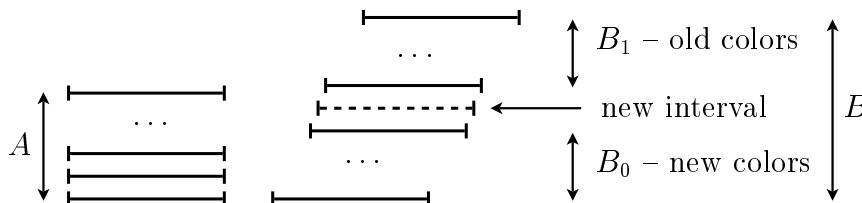
FIGURE 12. Construction of B = B_0 \cup B_1 .
