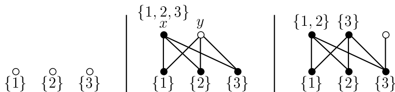
FIGURE 16. Spoiler forces 4 colors on the order of width 3. If Algorithm sticks to three colors, either x or y has only one color upon the arrival of y . In both cases Spoiler may present a point forcing the fourth color.
