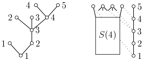
FIGURE 2. Strategy S(5) for Spoiler.
