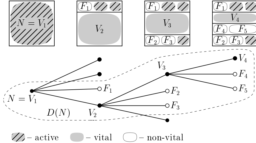
FIGURE 5. The tree-structure and the path of vital nodes in D(N) .
