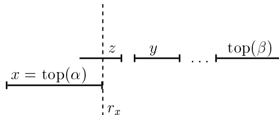
FIGURE 10. Each color is used on an interval containing r_x .
