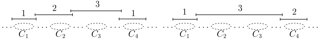
FIGURE 8. S(k + 1) : Algorithm has to use three different colors.
