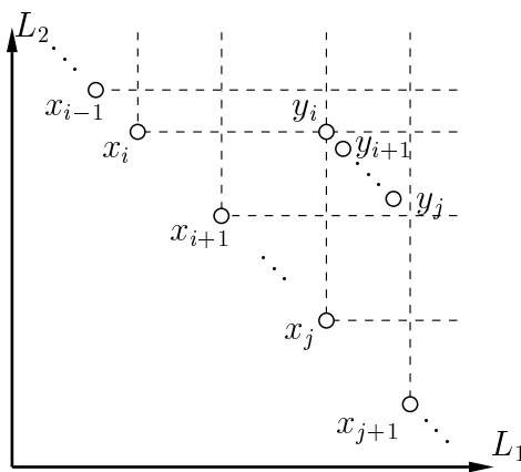
FIGURE 14. Combination of above i,j followed by left i,j .
