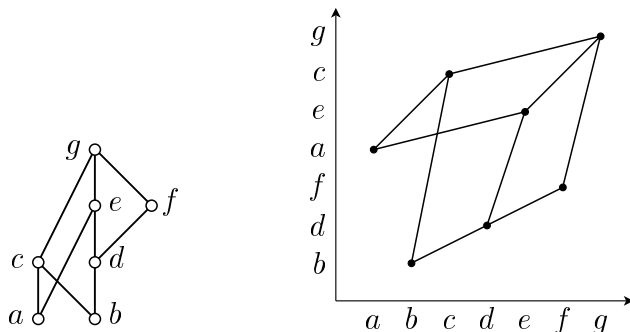
FIGURE 13. Poset embedded into a 2-dimensional grid.
