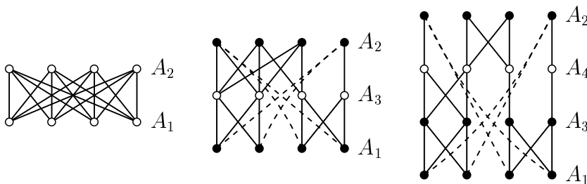
FIGURE 3. The first two moves of Spoiler in a regular game of width 4.
