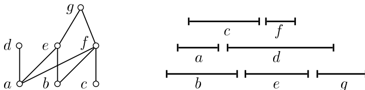
FIGURE 6. Interval order \mathbf{P} = (\{a, b, c, d, e, f, g\}, \leq) with its representation.
