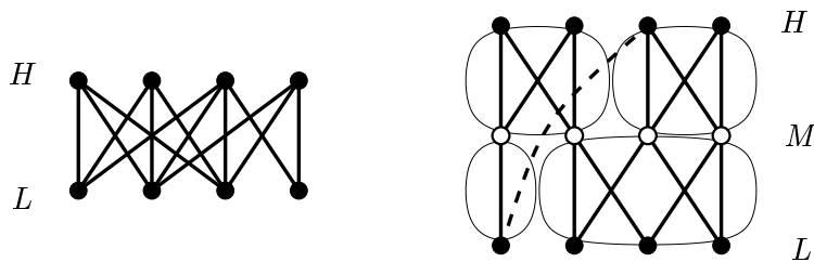
FIGURE 4. A node in the strong order (L, H) and its four sons in strong orders (L, M) and (M, H) .
