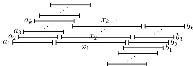
FIGURE 11. Strategy for Spoiler forcing Algorithm to use 2w - 1 chains on a semi-order of width w .
