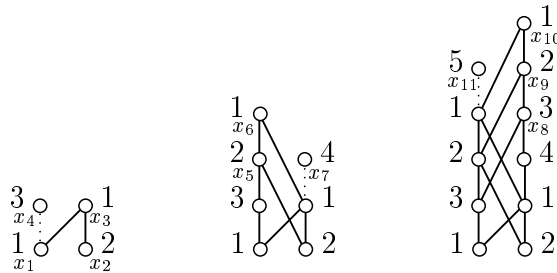
FIGURE 15. First-Fit forced to use 5 chains on an order of width 2.
