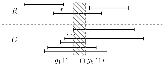
FIGURE 9. \gamma(r) \not\subseteq r' for all r' \in R - \{r\} .
