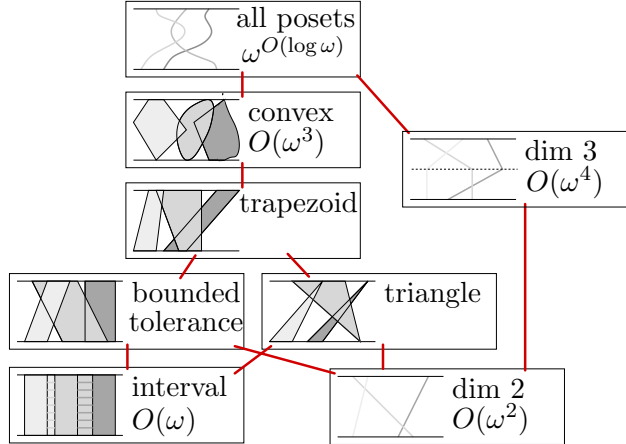
FIGURE 1. The containment order of some classes of graphs given by objects between two lines together with the performance guarantee for the best known on-line coloring algorithm (given the intersection representation as input).
