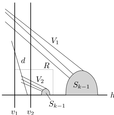
FIGURE 6. Strategy S_k consists of two calls of strategy S_{k-1} and the additional of an extra segment d . Algorithm A unavoidably uses k colors on the segments intersecting v_1 or on the segments intersecting v_2 .
