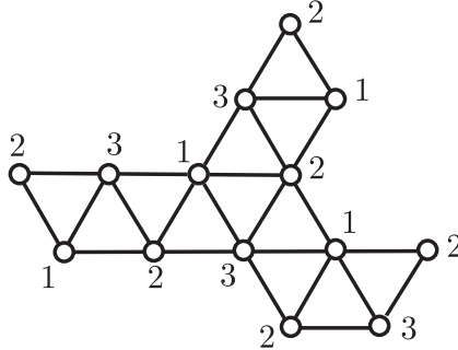
FIGURE 3. An Outerplanar Graph
