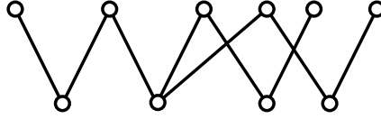
FIGURE 4. A Poset of Height 2
