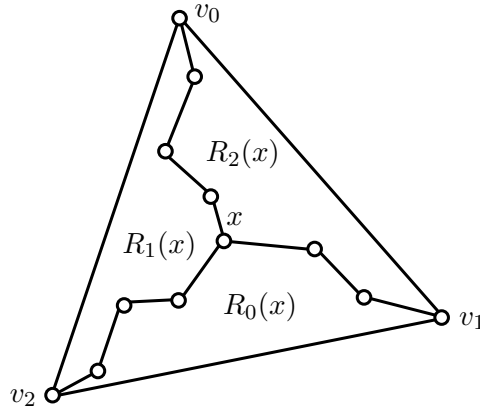
FIGURE 1. Schnyder Paths and Regions
