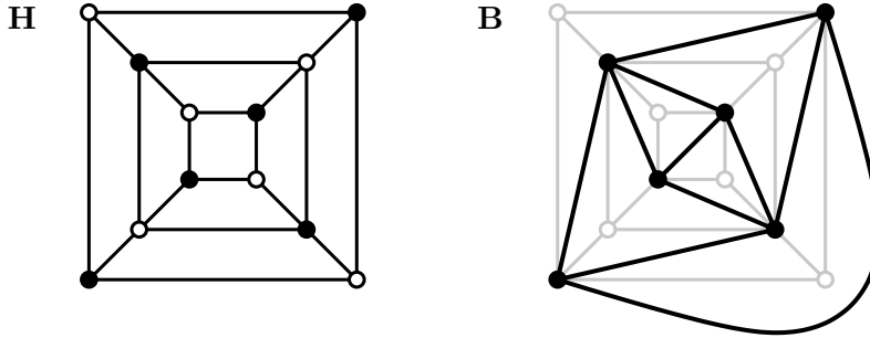
FIGURE 2. A Planar Bipartite Quadrangulation \mathbf{H} and its Associated Graph \mathbf{B} .
