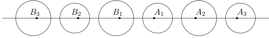
Fig. 1.24. Schottky uniformization of an M-curve.
