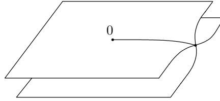
Fig. 1.5. Riemann surface of \sqrt{\lambda}
