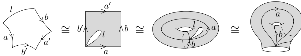
Fig. 1.13. Gluing a handle
