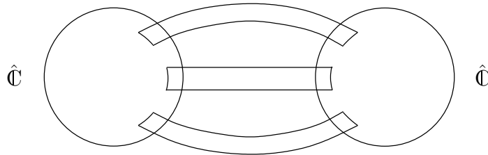
Fig. 1.6. Topological image of a hyperelliptic surface
