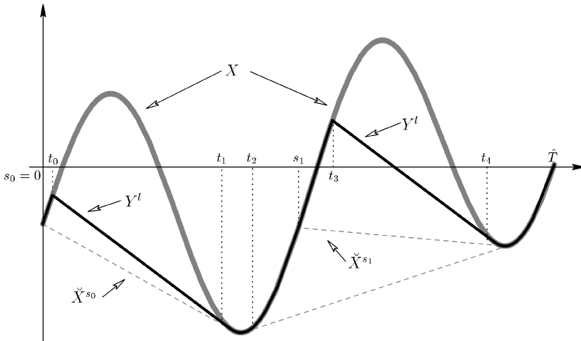
FIG. 2. A function X (thick grey line), the associated function Y^l for some fixed l (black line) and two convex envelopes \check{X}^{s_i} , i = 0, 1 , starting in (s_i, X(s_i)) , respectively (dashed grey lines).
