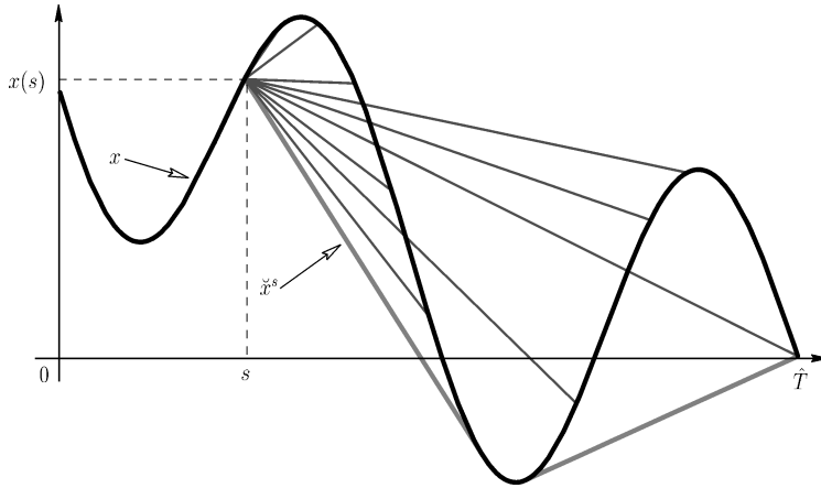
FIG. 1. A function x (thick black line), its convex envelope \check{x}^s (thick grey line), and various secants (thin lines) starting in (s, x(s)) .
